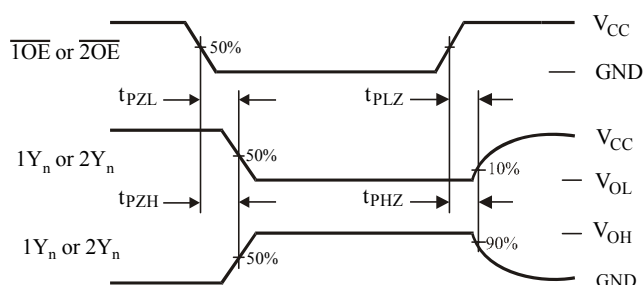
Figure 2. Switching Waveforms
